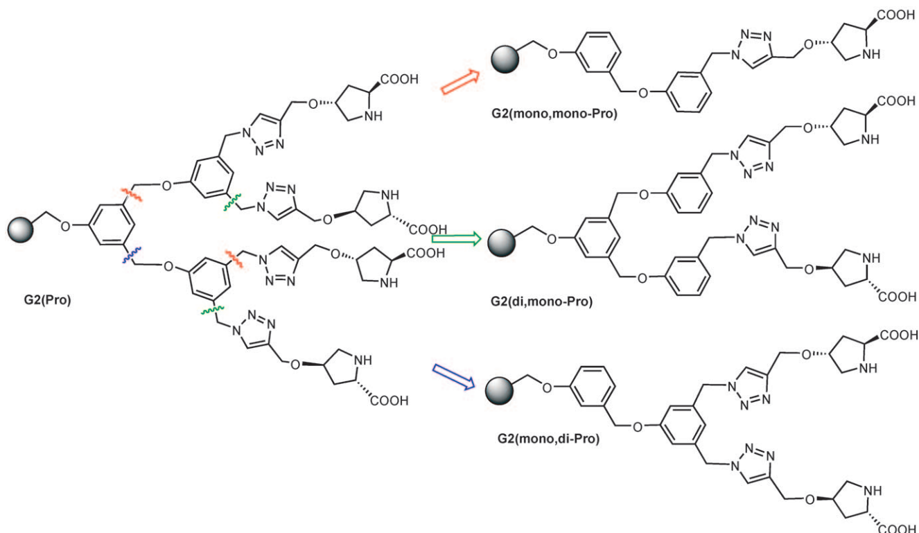
Scheme 2. Truncated spacer models of the G2 catalyst.
