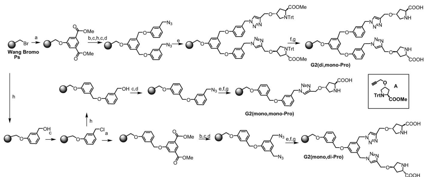
Scheme 3. Synthesis of the G2 catalyst models. Reagents and conditions: a) dimethyl 5-hydroxyisophthalate, LiH, TBAI, DMF, 60 °C, overnight; b) LiBH 4 , B(OMe) 3 , THF, 60 °C, overnight; c) PPh 3 , C 2 Cl 6 , THF, room temperature, overnight; d) NaN 3 , TBAI, DMF, 60 °C, 24 h; e) A , sodium ascorbate, CuSO 4 , DMF, 50 °C, overnight; f) 0.2% TFA in DCM, room temperature, 5 min; g) LiOH, THF/H 2 O, 40 °C, 4 h; h) 3-hydroxybenzyl alcohol, LiH, TBAI, DMF, 60 °C, overnight.
